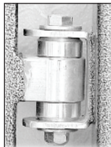
Slotted Yoke Allows For a 1/2" of Adjustment On Each Hinge.
